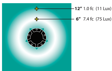
SL-20-SMM Light Distribution
