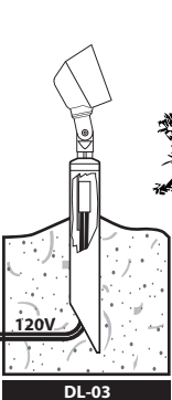
DL-03 OPTIONAL COMMERCIAL (FA-26 75) 120V
