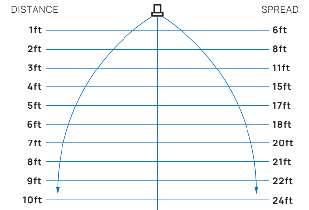
Light Distribution (Single Fixture) 8 inches from grade
