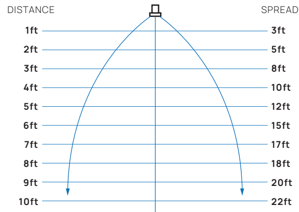
Light Distribution (Single Fixture) 6 inches from grade
