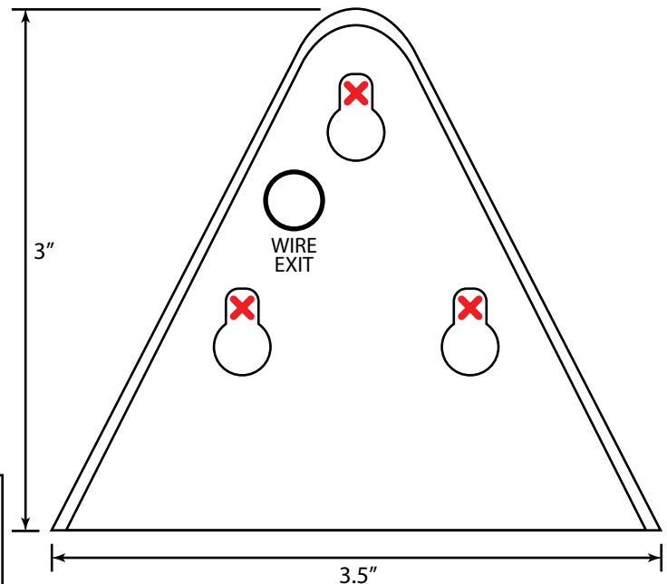
MOUNTING TEMPLATE "X" inside key holes mark location of screw(s)
