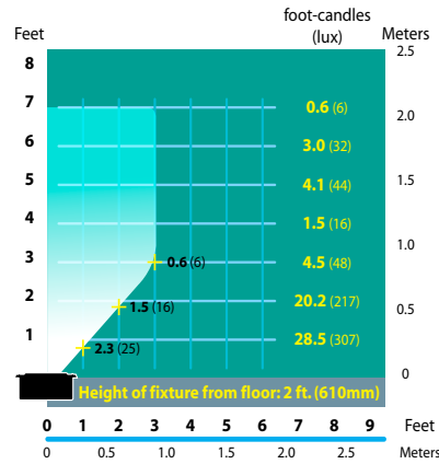
SL-04 Half Spread Photometrics
