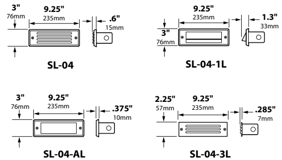
SL-04: Mounting Holes on all models 7-1/2" on center
