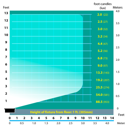
SL-04-AL Half Spread Photometrics
