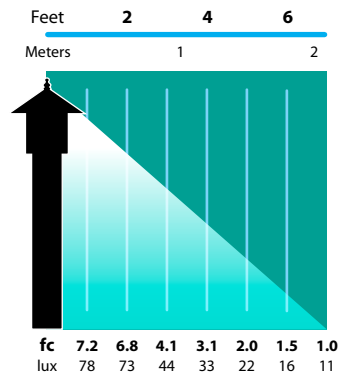
AL-09 Half Spread Photometrics 14 ft. (4.3m) diameter
