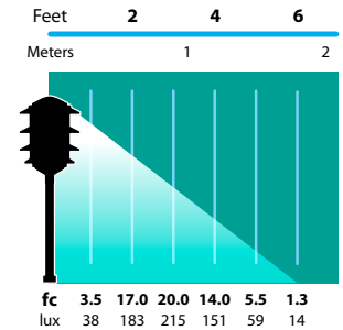
AL-03-4T Half Spread Photometrics 12 ft. (3.7m) diameter
