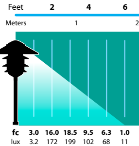
AL-03-4T-10 Half Spread Photometrics 12 ft. (3.7m) diameter
