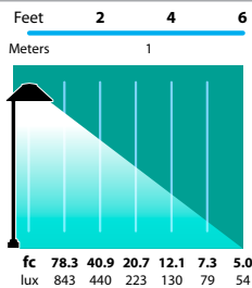
PL-01 Half Spread Photometrics 12 ft. (3.7 m) diameter
