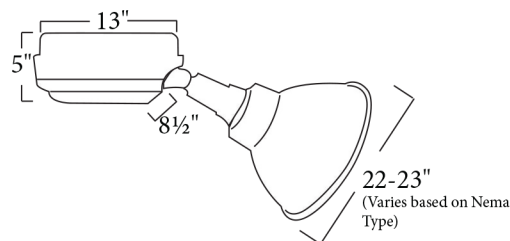
Shown with SP50PT Tenon Adaptor (Ordered Separately)
