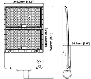
Slipfitter Mount
