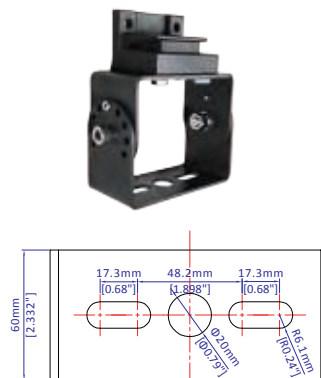
Trunnion Mount
