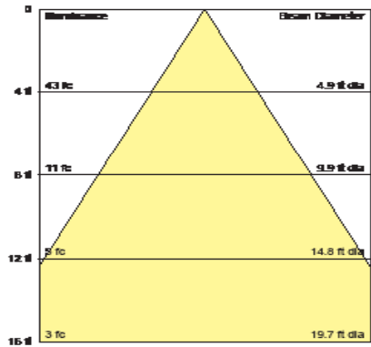
WLARFL36CWL 36W WLAR LED Flood Optic Color Temperature: 5,900 K
