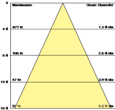
WLARFL36CWL 36W WLAR LED Spot Optic Color Temperature: 5,900 K
